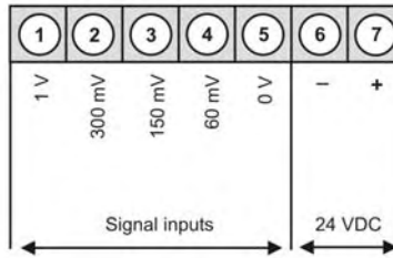
Type M3-7VR5A.0002.770AD with a supply of 24 VDC
