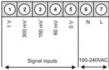
Type M3-7VR5A.0002.S70AD with a supply of 100-240 VAC
