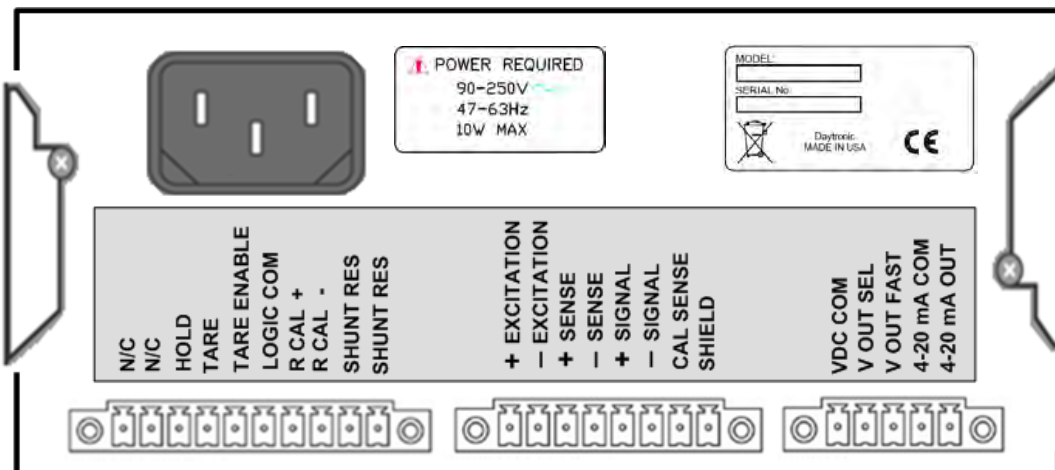
Rear Panel View - screw terminal connectors, provided
